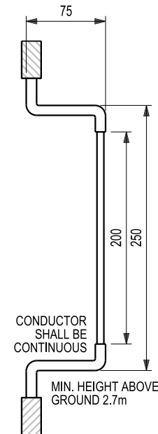
DETAIL A
